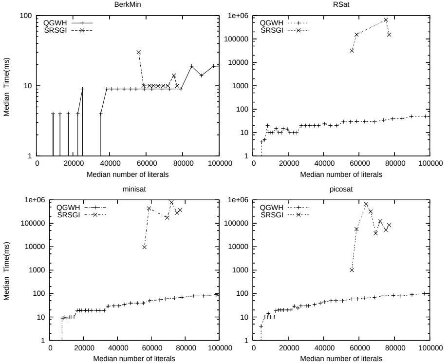
Fig. 7. Empirical hardness of SRSOI ( m=24 , q=193 , n=20 ) and QGWH (order 20) for complete solvers. Size of the instances is used as comparison criteria. Some points are missing from the SRSOI plots due to time out. Notice the logarithmic time scale.
