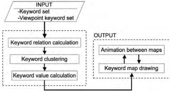
Fig. 1. Structure of animation interface
