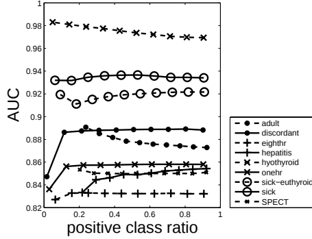
Fig. 4. Naive Bayes (with original class distribution or with under-sampling) performs well except on the Eighthtr where cost-based sampling performs significantly better
